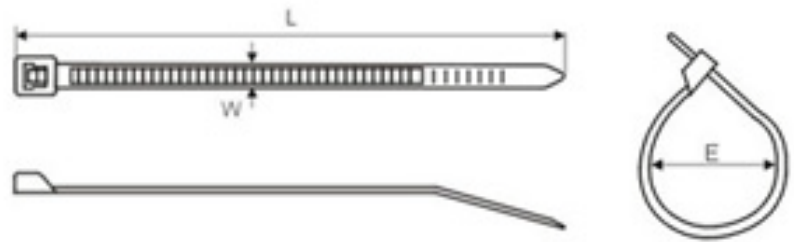
Self-locking nylon cable ties
